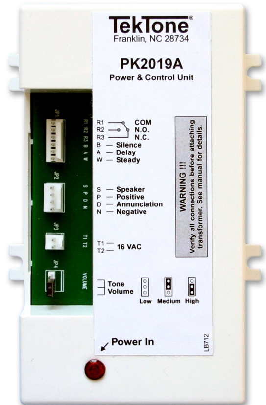
PK2019A Power & Control Unit
