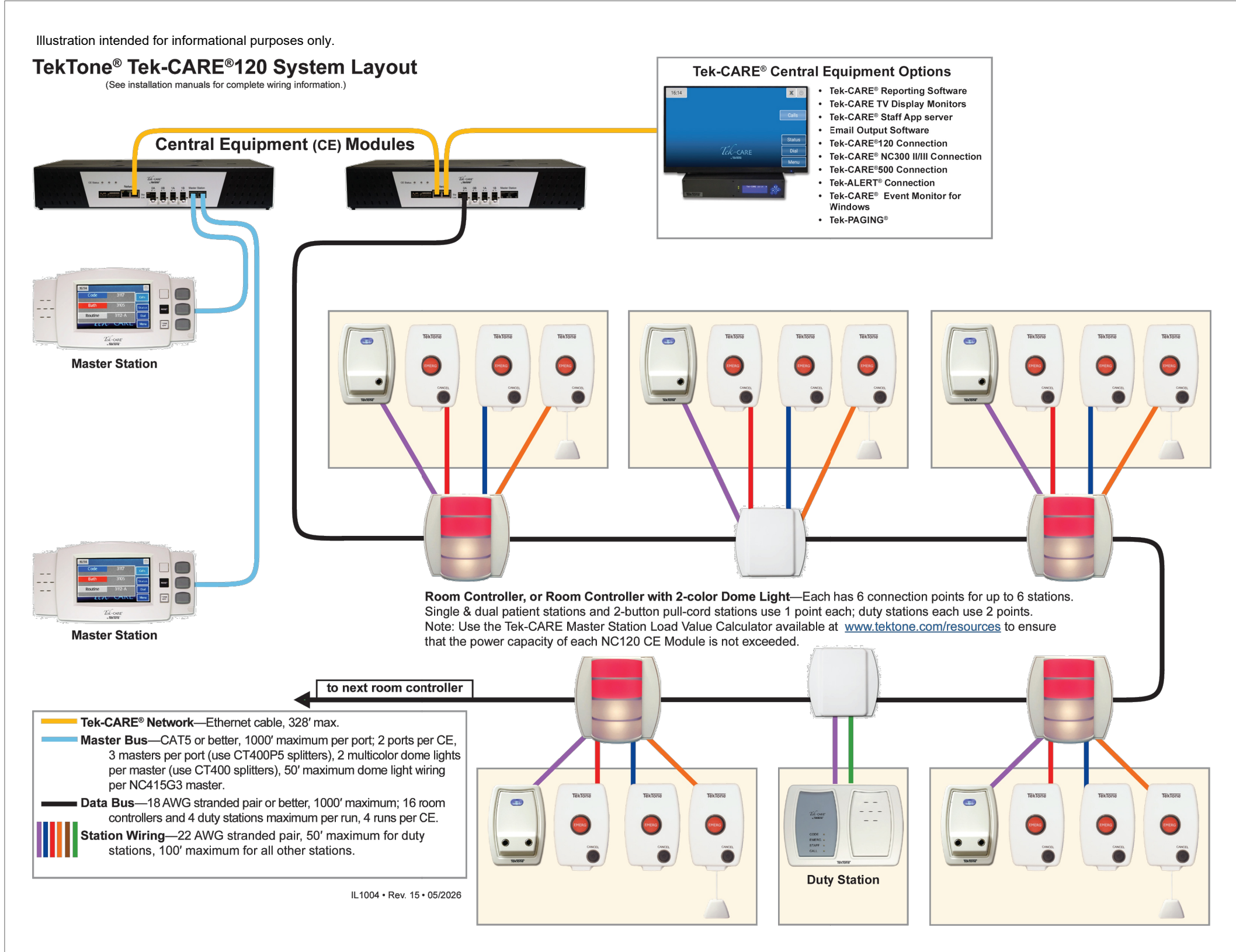
Tek-CARE 120 STANDARD SYSTEM LAYOUT SCALE: NONE
