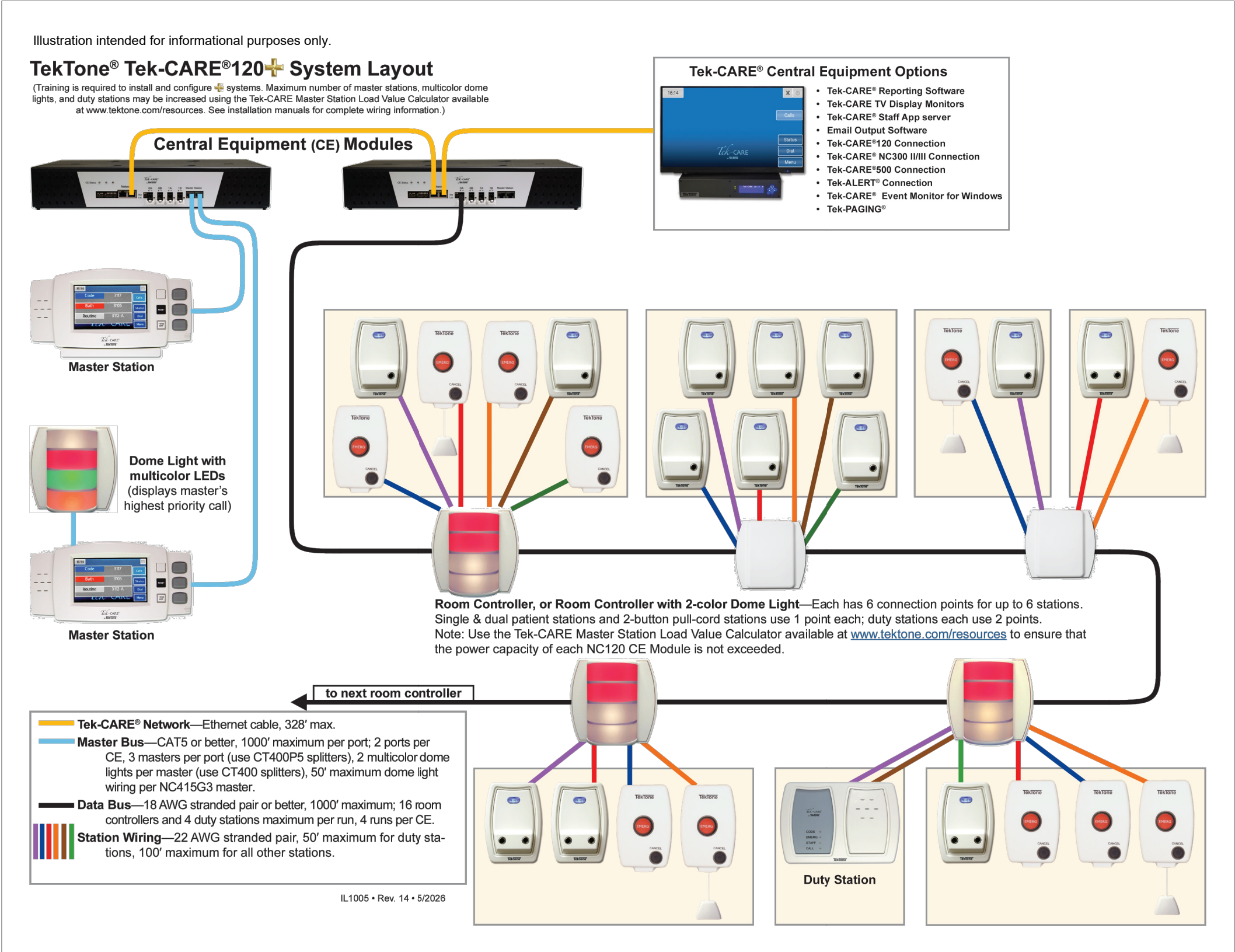
Tek-CARE 120+ SYSTEM LAYOUT SCALE: NONE
